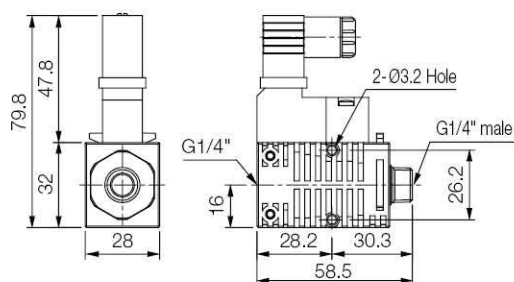
[DIN type]
