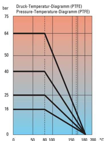
Druck - Temperatur - Diagramm / Pressure - Temperature - Diagram
